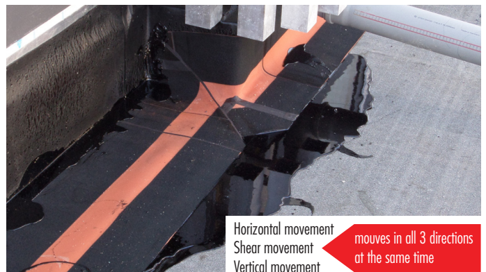
Hot applied liquid bitumen
