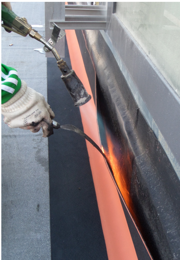
Torch applied bitumen membrane
